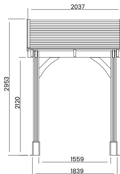
VIEW FROM FRONT
